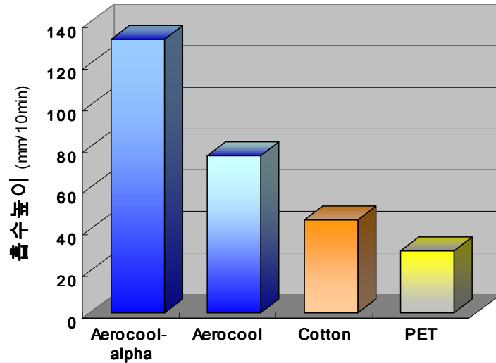
Hygroscopicity (by JIS L 1096)
